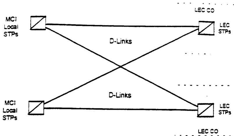
FIGURE 10. D-LINK Interface
