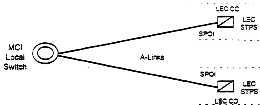
Figure 6. A-Link Interface
