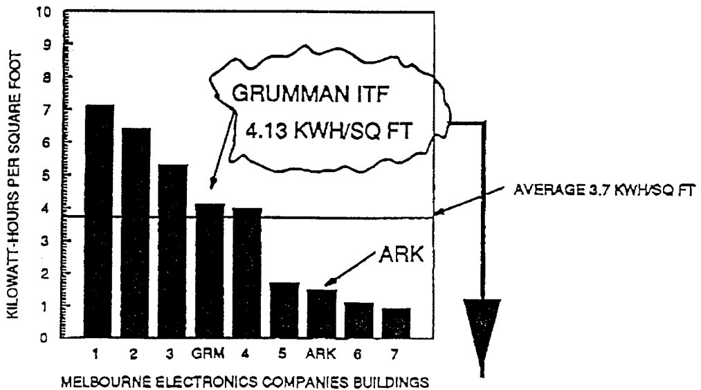
MELBOURNE ELECTRONIC COMPANIES COMPARISON KILOWATT HOURS PER SQUARE FOOT
