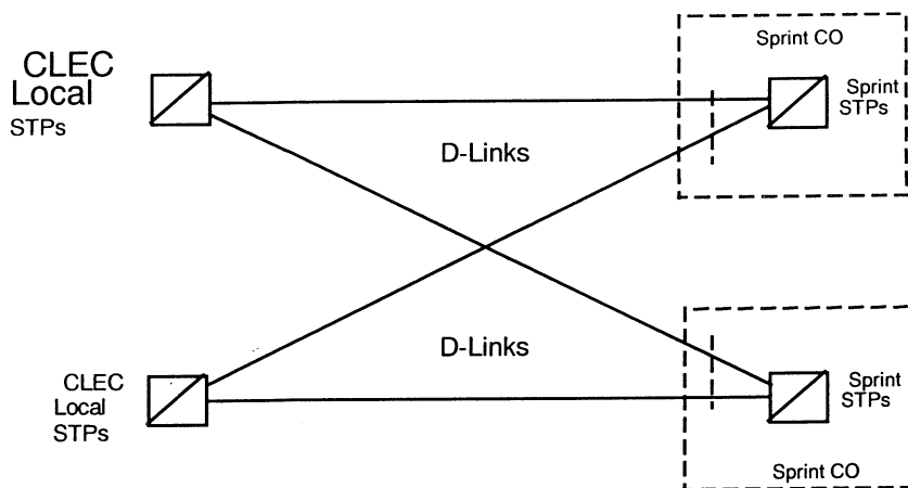
Figure 4. D-Link Interface
