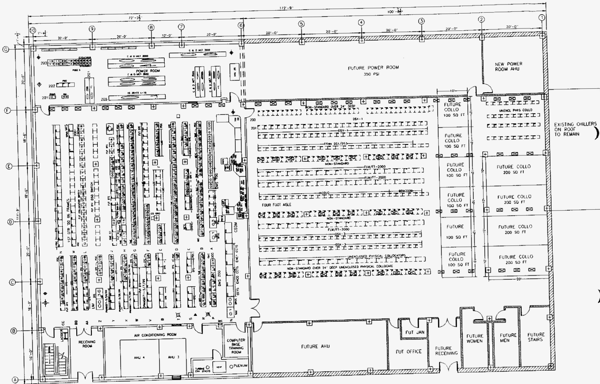
M6506 NORTH DADE GOLDEN GLADES SECOND FLOOR PLAN 2001 BUILDING ADDITION PSC WAIVER ITEM 4 G-H PAGE 2
