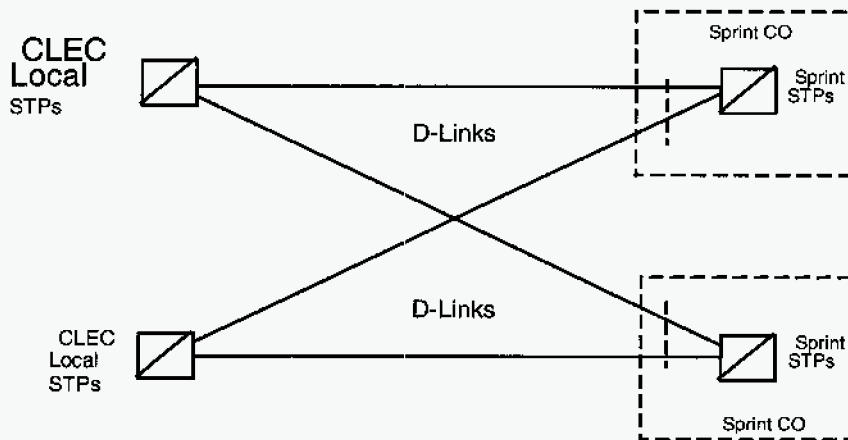
Figure 4. D-Link Interface
