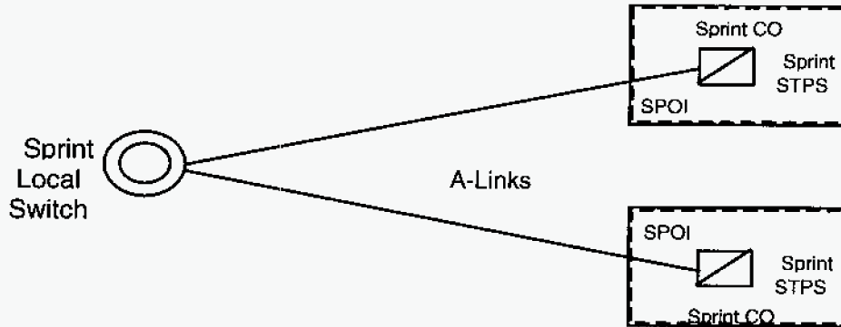
Figure 3. A-Link Interface
