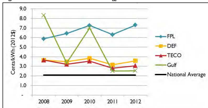
Figure 5.1. Levelized Cost of Saved Energy: Florida Utilities versus National Average. 21
