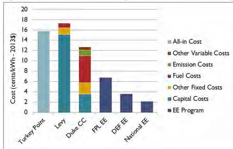
Figure 2.3 Cost of Generation Technologies versus the Cost of Saved Energy
