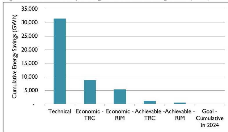
Figure 4.1 FPL Efficiency Savings at Various Screening Levels (GWh) 17
