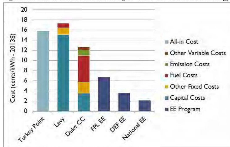
Figure 5.2. Cost of Generation Technologies versus the Cost of Saved Energy
