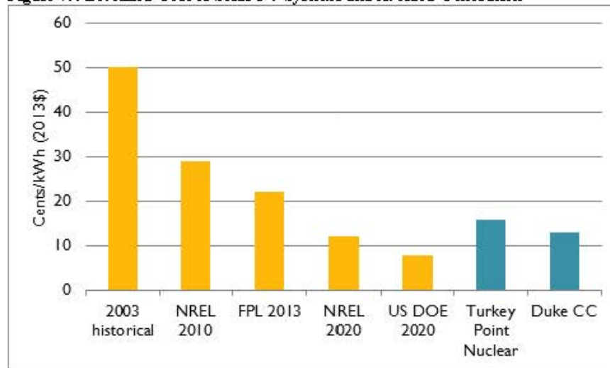
Figure 7.4 Levelized Cost of Solar PV Systems and Avoided Generation
