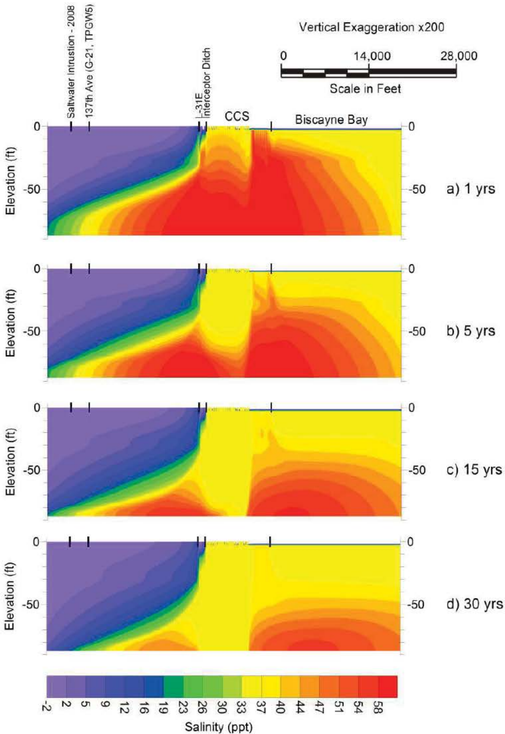
Figure 5. Demonstrative 19. TetraTech (2013b), Modeled Salinity at Specific Times During Proposed CCS Salinity Reduction
