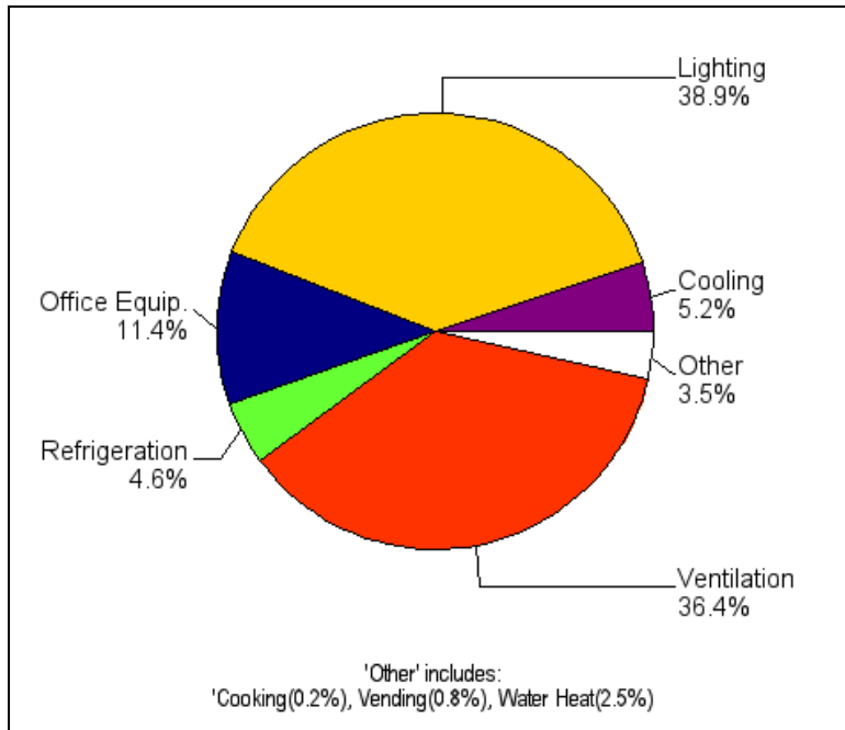
Figure 3-29: Estimated Breakdown of Total Technical Potential for Commercial Winter System Peak Demand Savings in Gulf Power by End Use (136 MW)
