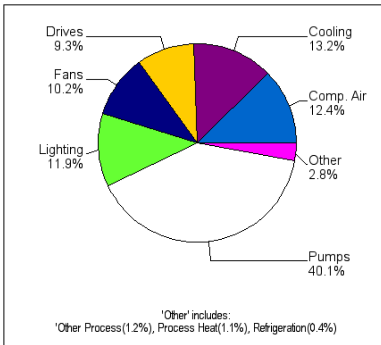
Figure 3-34: Estimated Breakdown of Total Technical Potential for Industrial Summer System Peak Demand Savings in Gulf Power by End Use (15 MW)
