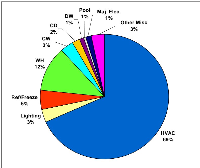
Figure 3-11: Estimated Breakdown of Total Residential Winter Peak Demand in Gulf Power (Excluding losses) by End Use (1,270 MW)
