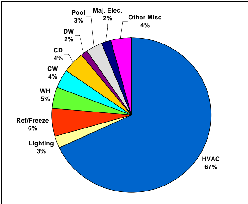
Figure 3-10: Estimated Breakdown of Total Residential Summer Peak Demand in Gulf Power (Excluding losses) by End Use (1,150 MW)
