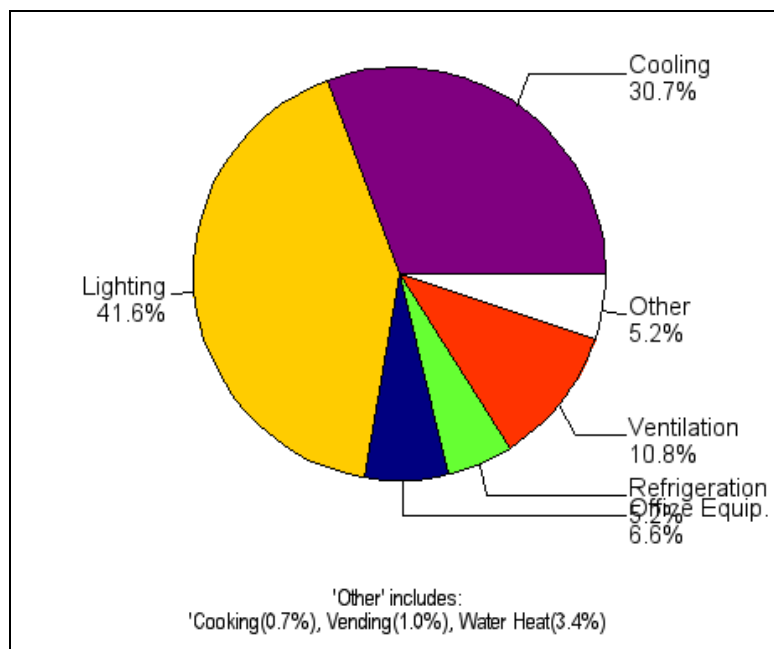
Figure 3-27: Estimated Breakdown of Total Technical Potential for Commercial Energy Savings in Gulf Power by End Use (1,210 GWh)
