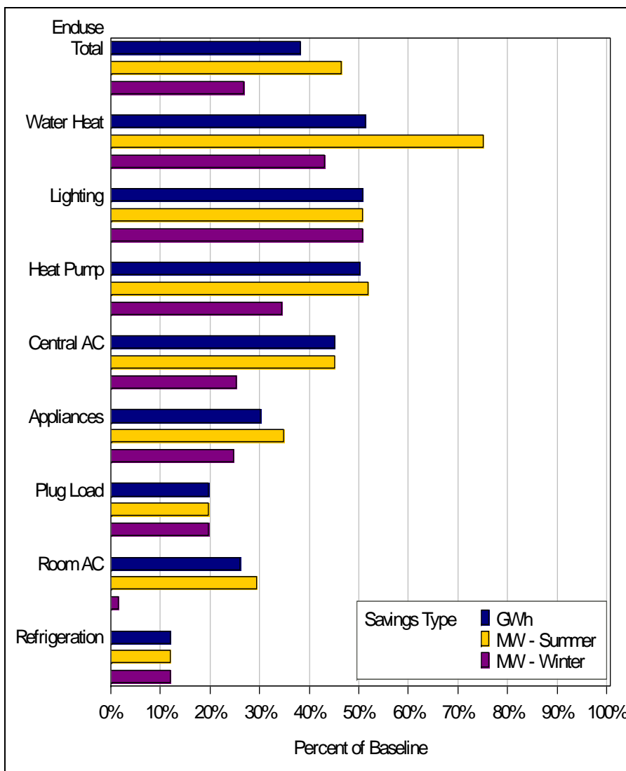
Figure 3-24: Total Technical Potential for End-use Energy and Peak Demand Savings in the Residential Sector Compared to Baseline Energy Consumption and Peak Demand in Gulf Power
