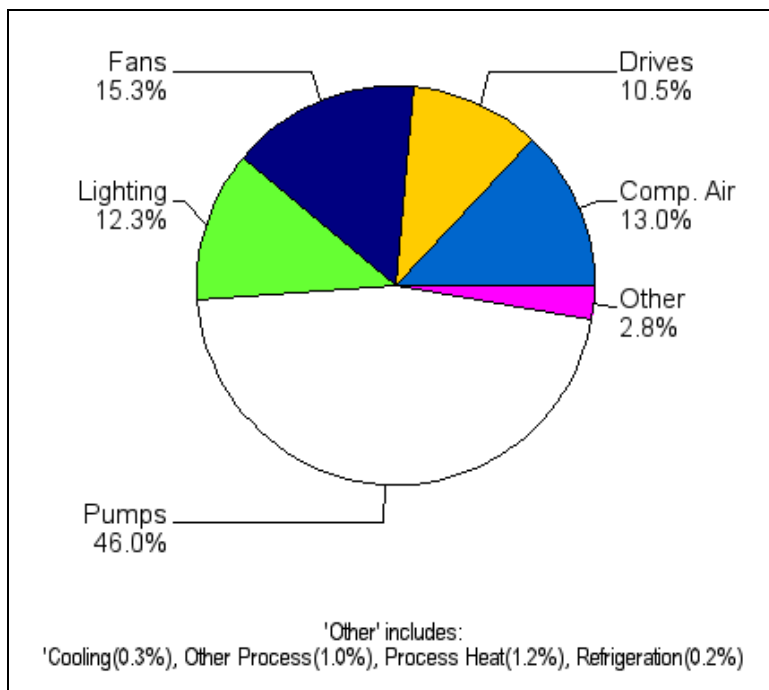
Figure 3-35: Estimated Breakdown of Total Technical Potential for Industrial Winter System Peak Demand Savings in Gulf Power by End Use (20 MW)
