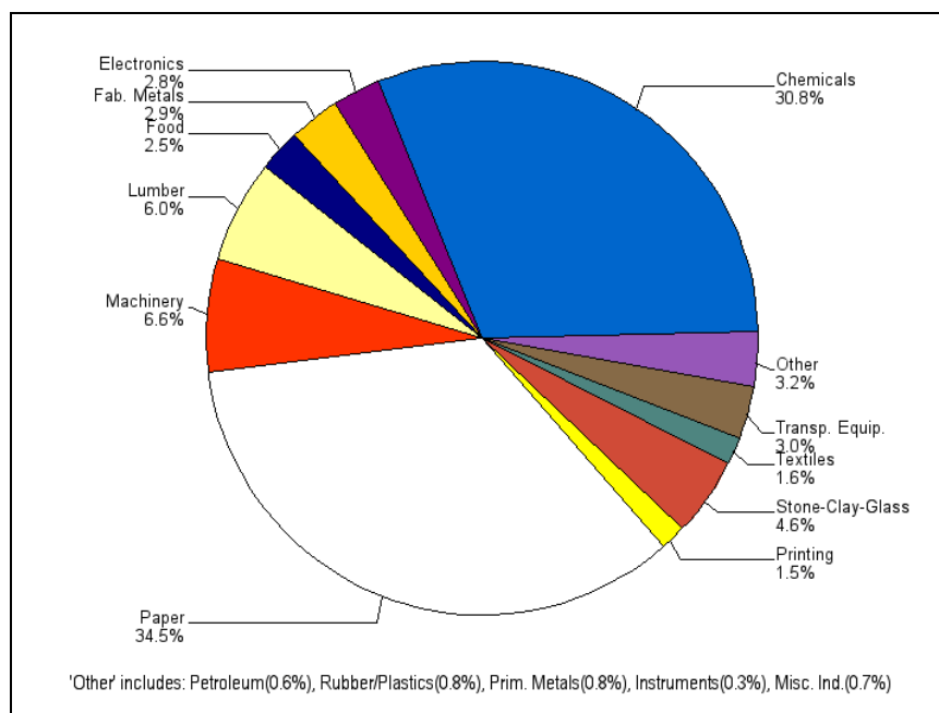
Figure 3-32: Estimated Breakdown of Total Technical Potential for Industrial Energy Savings in Gulf Power by Subsector (167 GWh)
