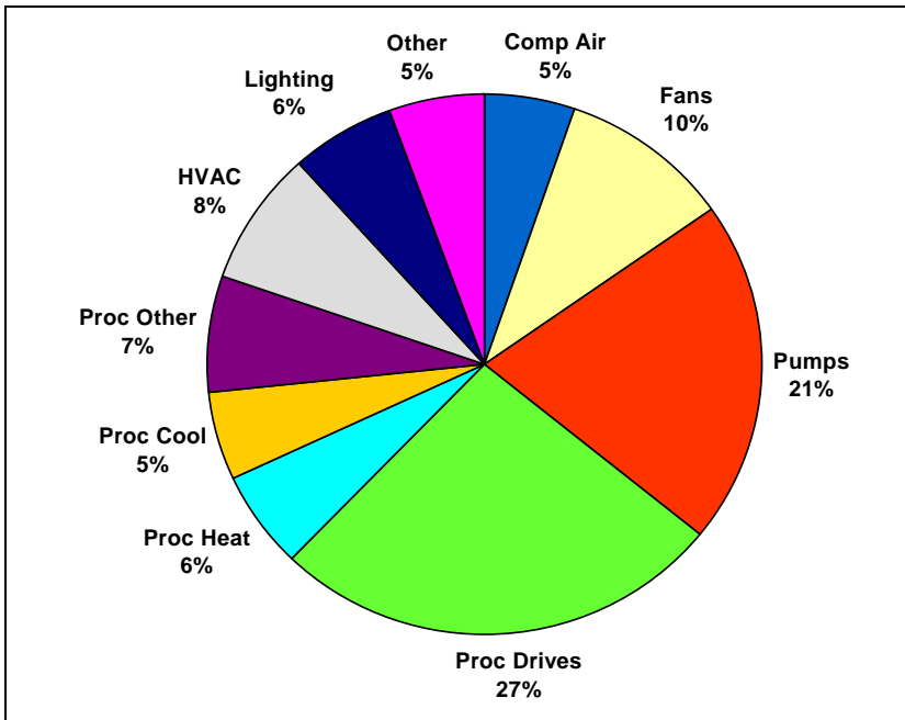
Figure 3-17: Estimated Breakdown of Total Annual Industrial Electricity Sales in Gulf Power (Excluding losses) by End Use (886 GWh)
