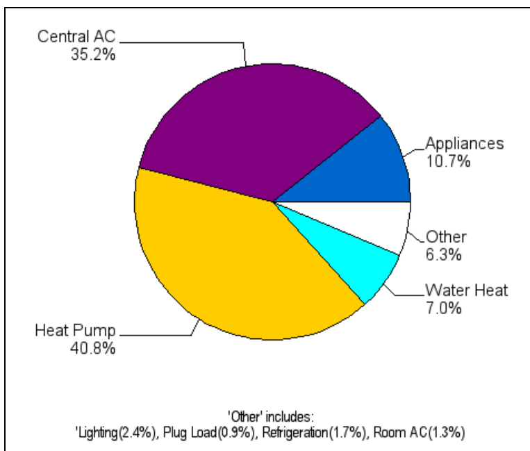
Figure 3-22: Estimated Breakdown of Total Technical Potential for Residential Summer System Peak Demand Savings in Gulf Power by End Use (534 MW)
