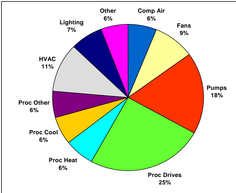
Figure 3-18: Estimated Breakdown of Total Industrial Summer Peak Demand in Gulf Power (Excluding losses) by End Use (96 MW)
