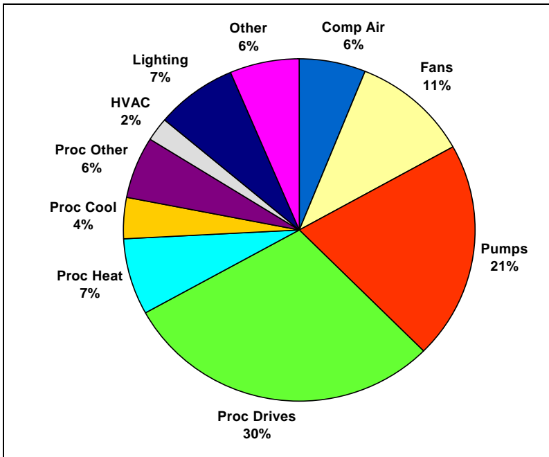
Figure 3-19: Estimated Breakdown of Total Industrial Winter Peak Demand in Gulf Power (Excluding Losses) by End Use (108 MW)
