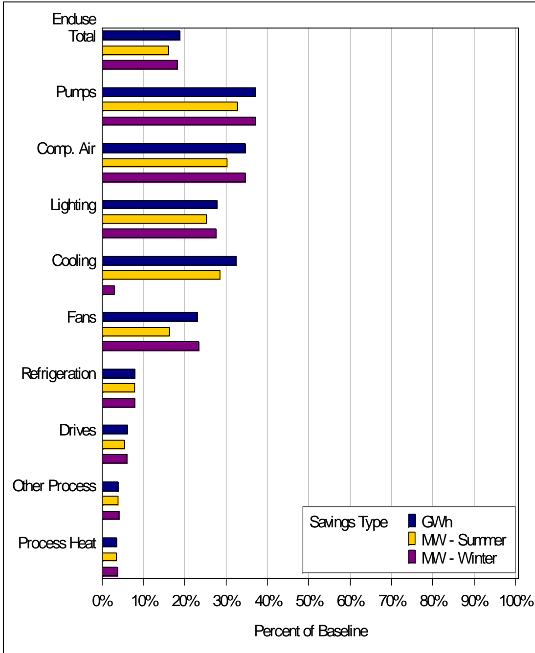
Figure 3-36: Total Technical Potential for End-use Energy and Peak Demand Savings in the Industrial Sector Compared to Baseline Energy Consumption and Peak Demand in Gulf Power
