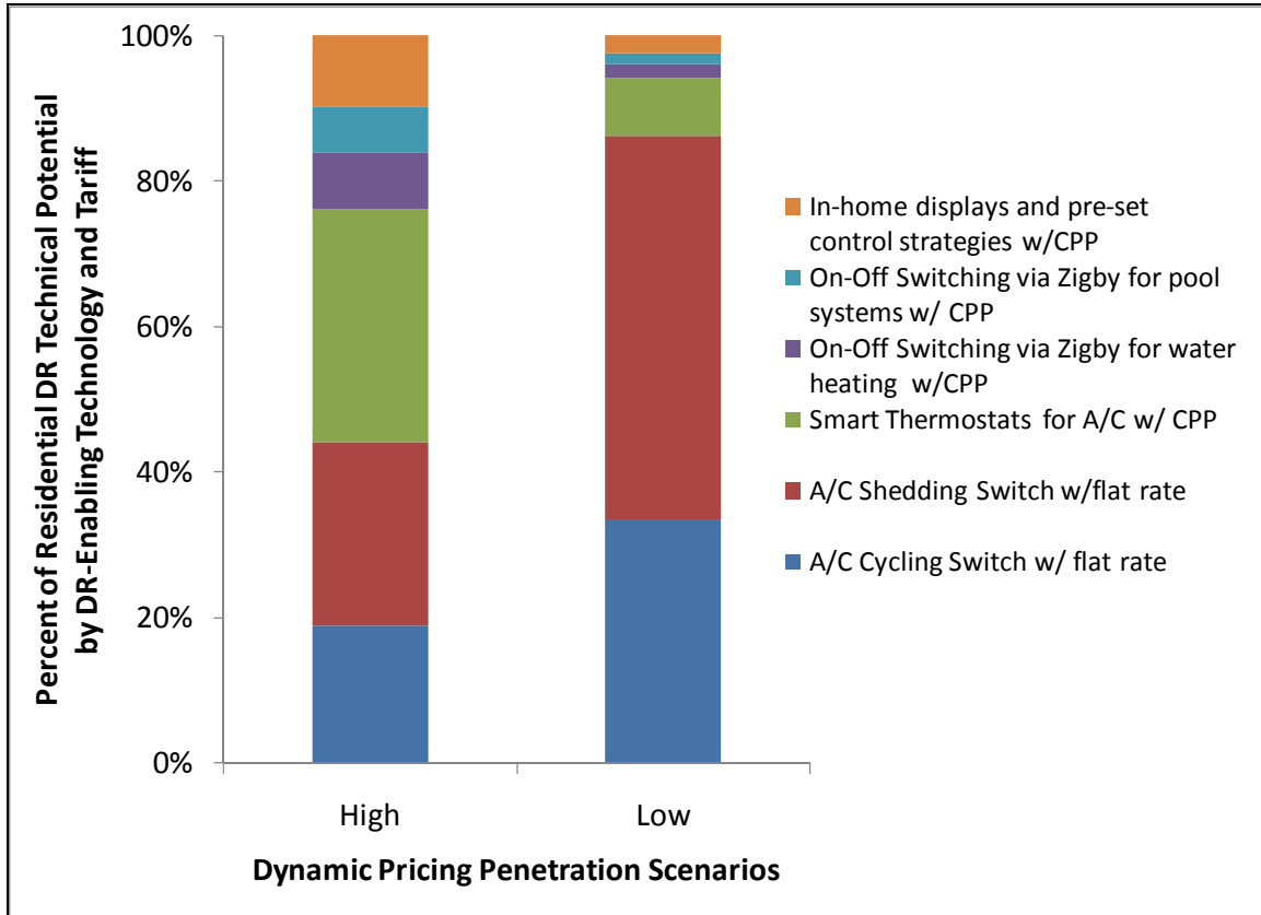
Figure 4-3: Composition of DR Technical Potential for Residential Customers in Gulf Power by Control Technology and Tariff in the “High” and “Low” Scenarios (Summer Peak Savings)
