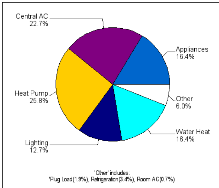
Figure 3-21: Estimated Breakdown of Total Technical Potential for Residential Energy Savings in Gulf Power by End Use (1,968 GWh)
