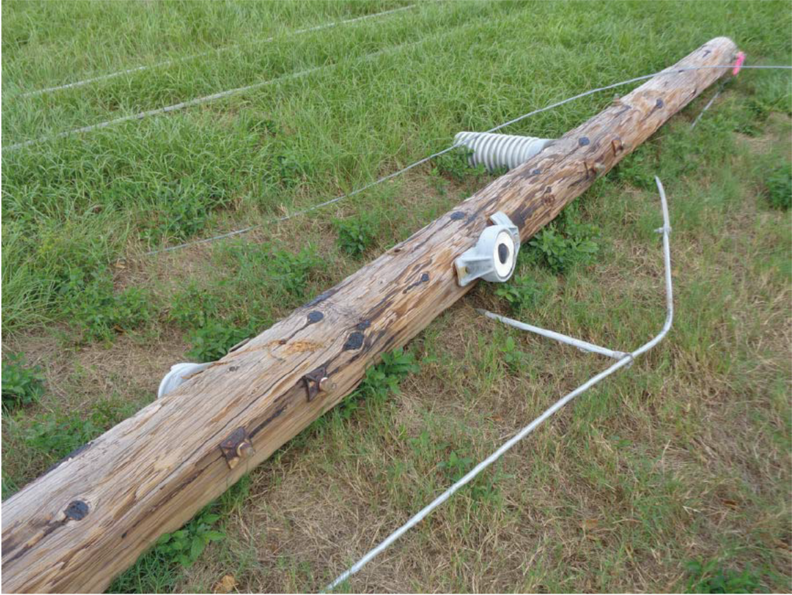
Wood pole AD-22 insulator damage. Looking northwest.
