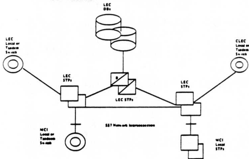
Figure 8. SS7 Network Interconnection
