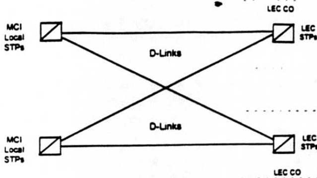
FIGURE 10. D-LINK Interface
