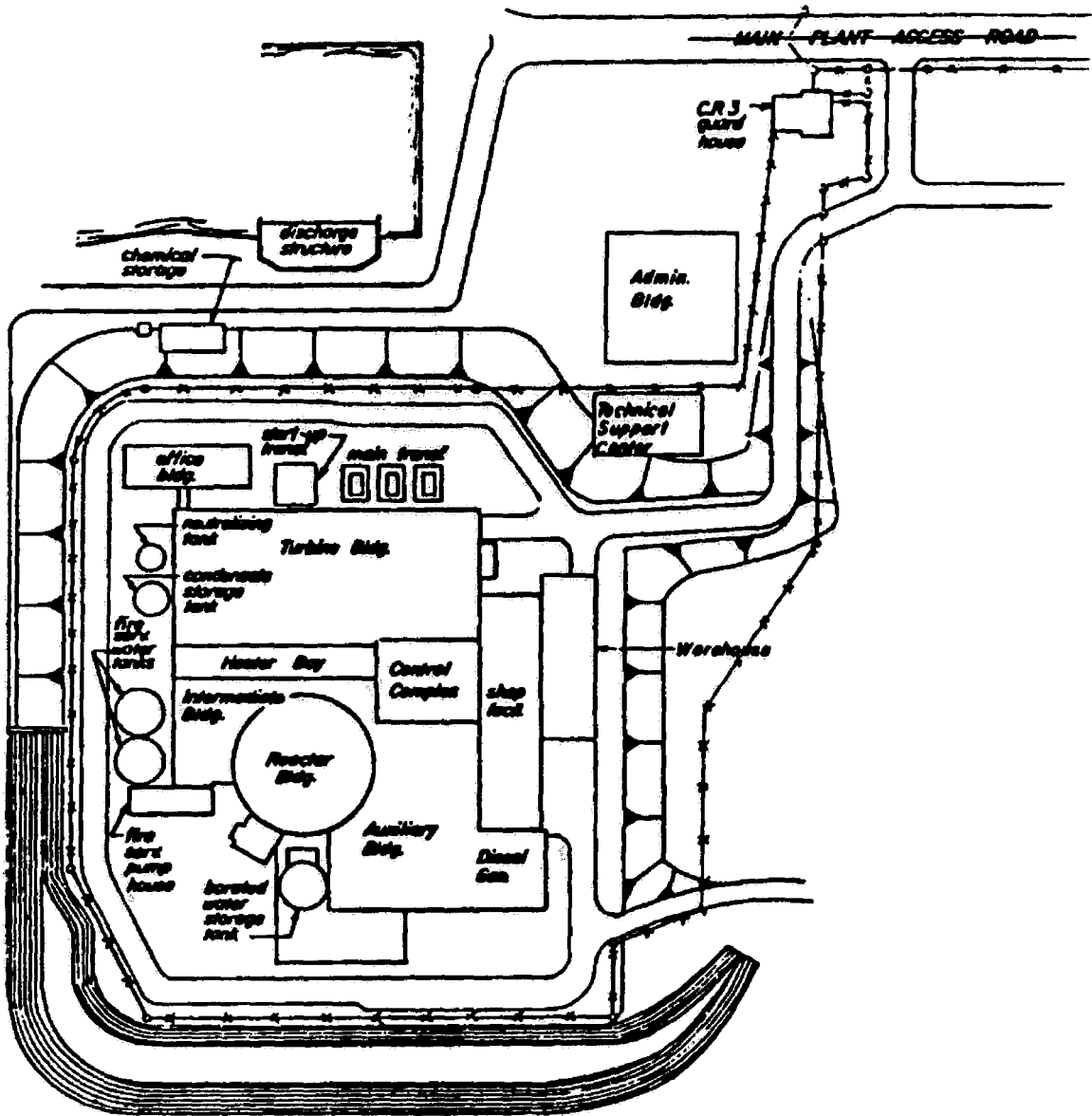
FIGURE 2.1 GENERAL ARRANGEMENT OF THE CRYSTAL RIVER PLANT - UNIT 3
