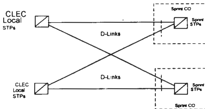
Figure 4. D-Link Interface
