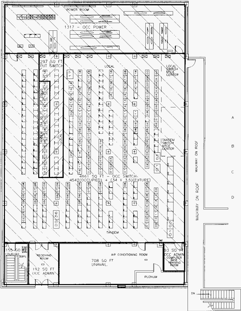
NORTH DADE GOLDEN GLADES SECOND FLOOR PLAN PSC WAIVER ITEM 4 A-F PAGE 4
