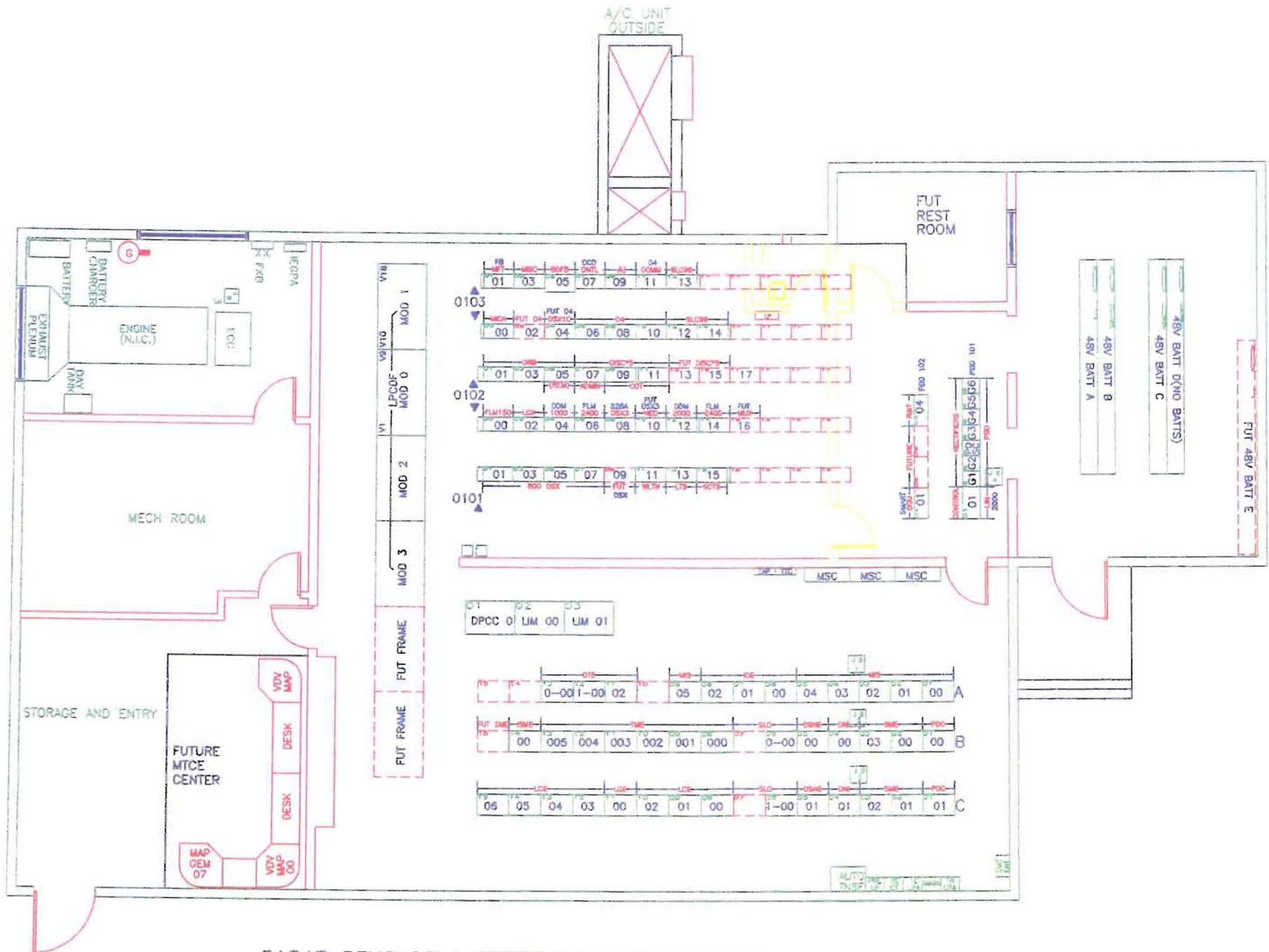
31347 PENSACOLA PERDIDO BAY FLOOR PLAN PSC WAIVER ITEM 4 G-H PAGE 1 (FUTURE)
