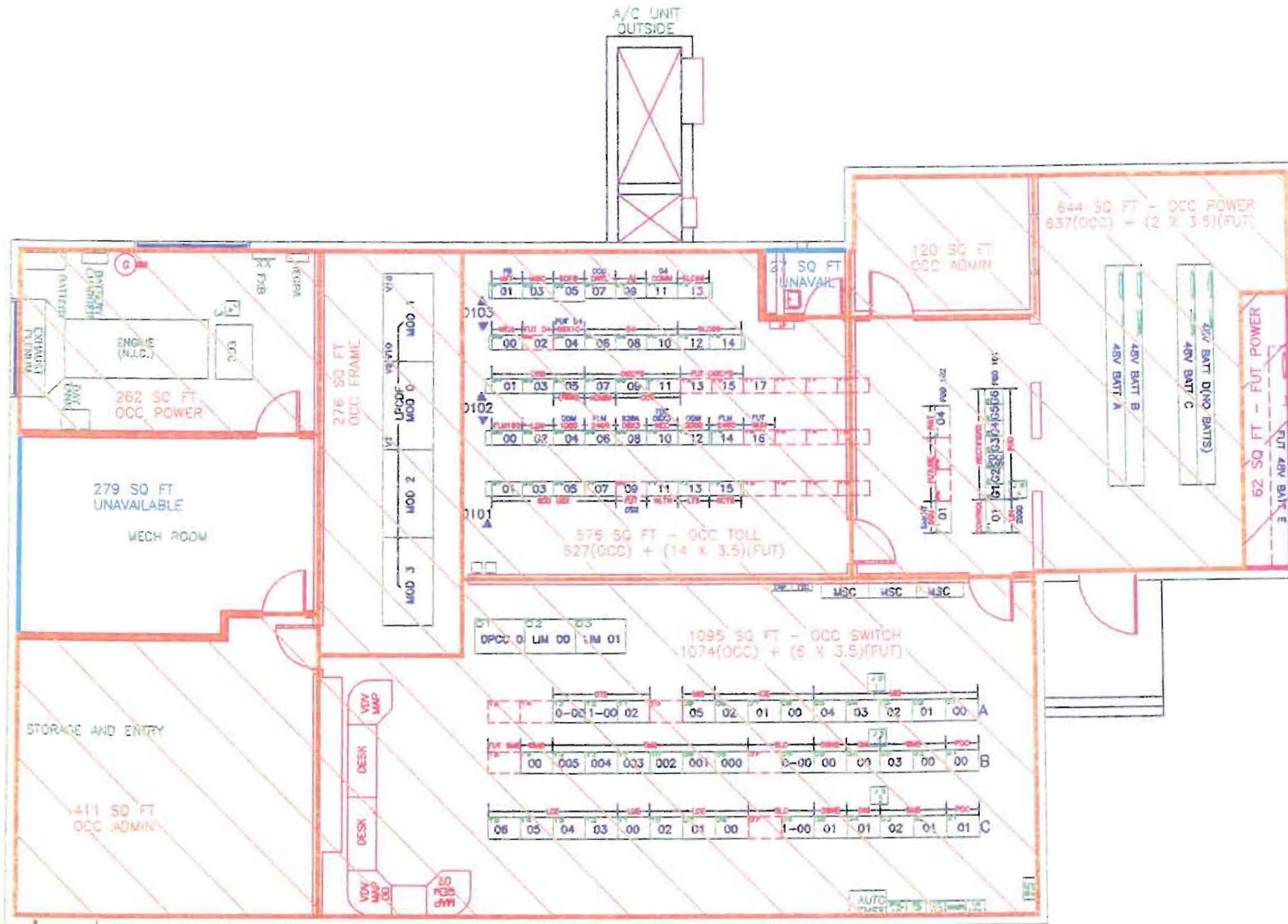
31347 PENSACOLA PERDIDO BAY FLOOR PLAN PSC WAIVER ITEM 4 A-F PAGE 2
