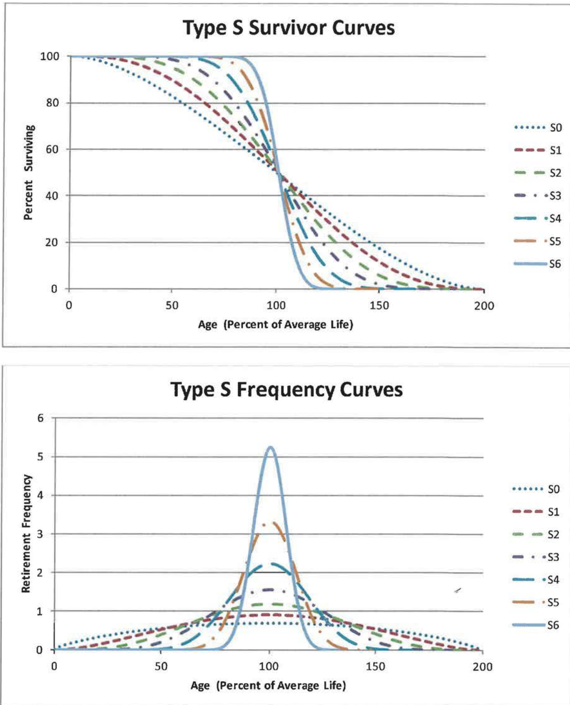
Figure 25: Type S Survivor and Frequency Curves
