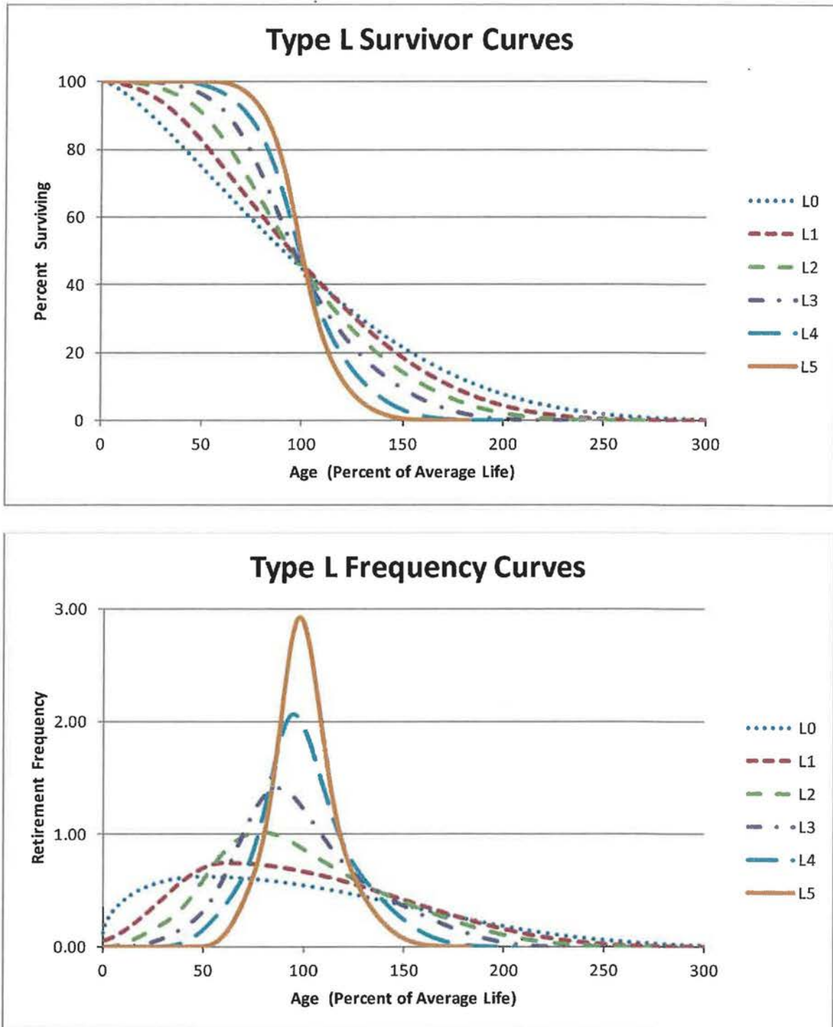
Figure 24: Type L Survivor and Frequency Curves
