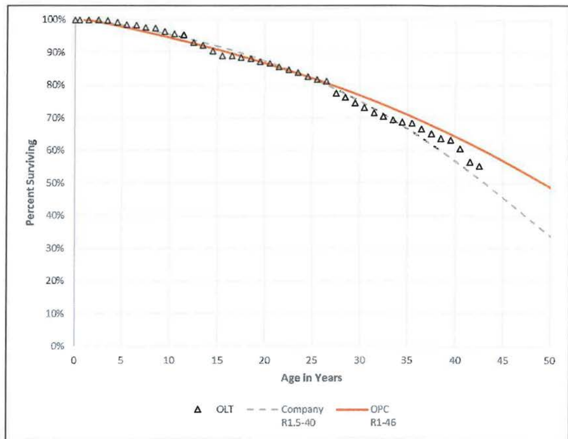
Figure 17: Account 368 – With Relevant OLT Curve
