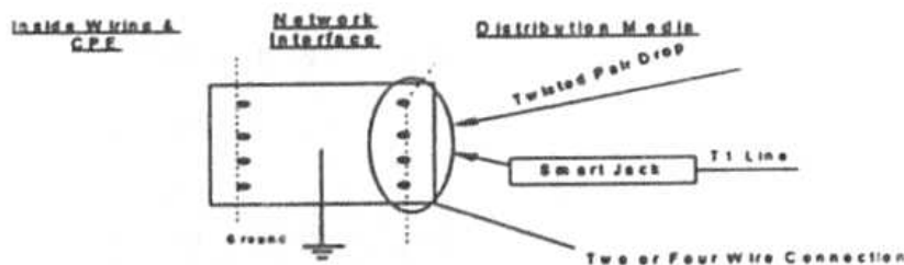
Figure 1 - Network Interface Device
