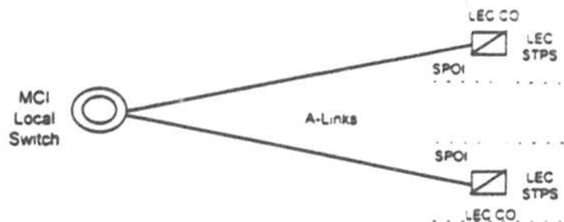
Figure 6. A-Link Interface
